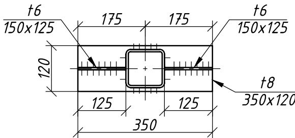
1-1, 2-2
